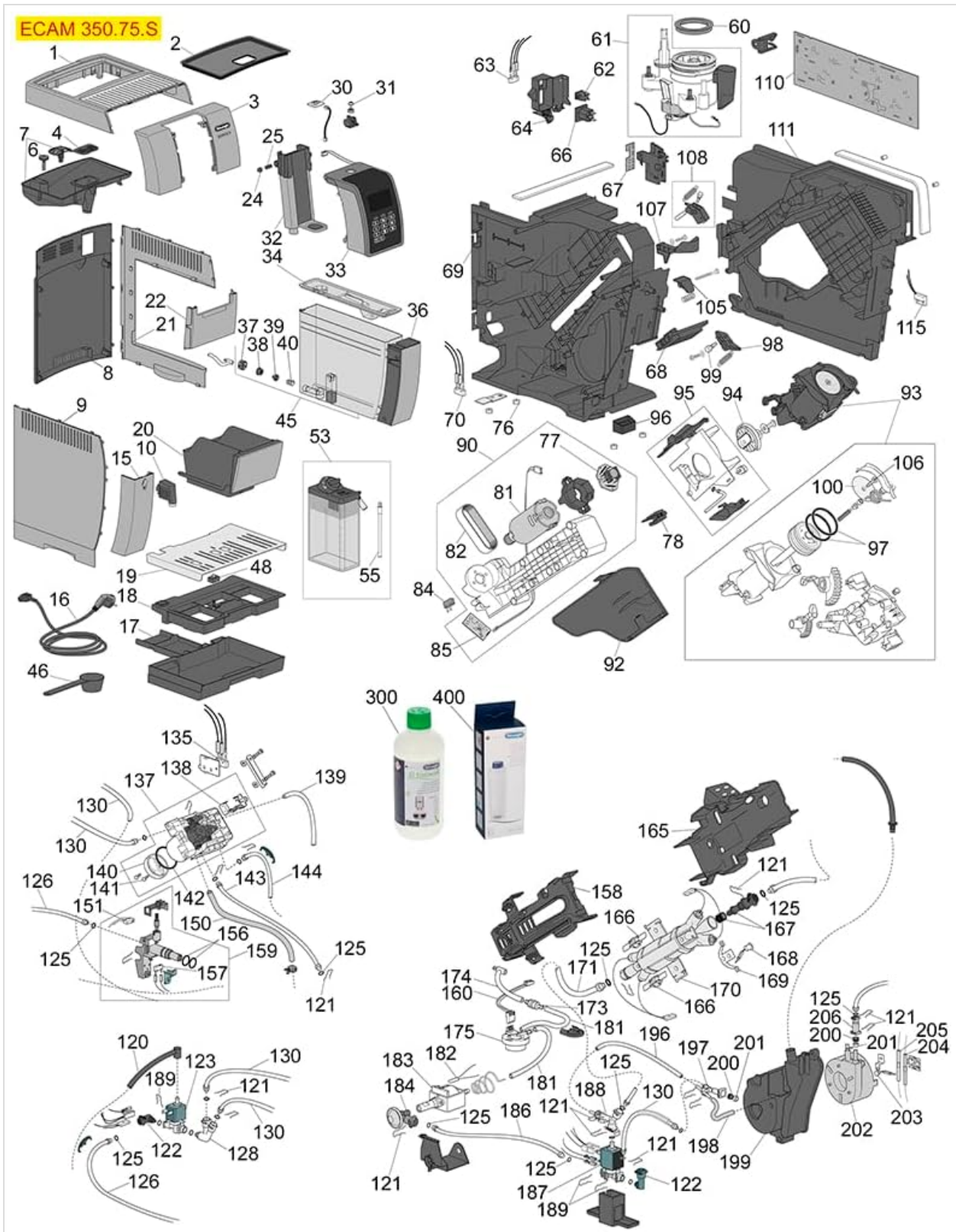
Figure 2: An exploded diagram illustrating various internal components of a DeLonghi coffee maker, including the boiler and filter assembly, with numbered parts for identification. Refer to your specific machine's service manual for exact part locations.
