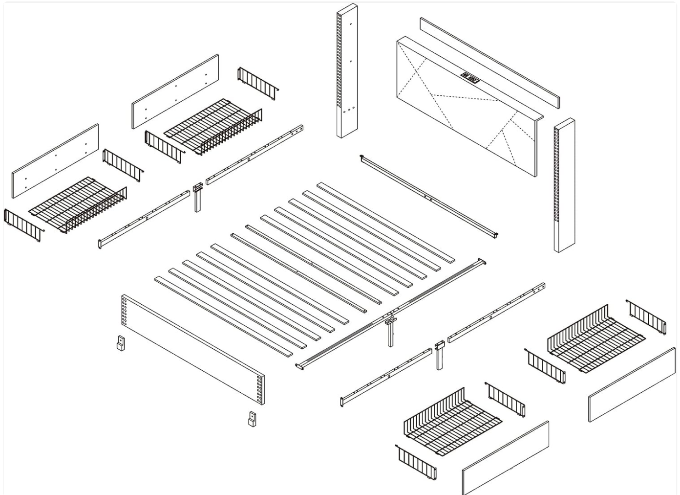
Image: Details of the one-click slat installation and sturdy metal frame connections.
