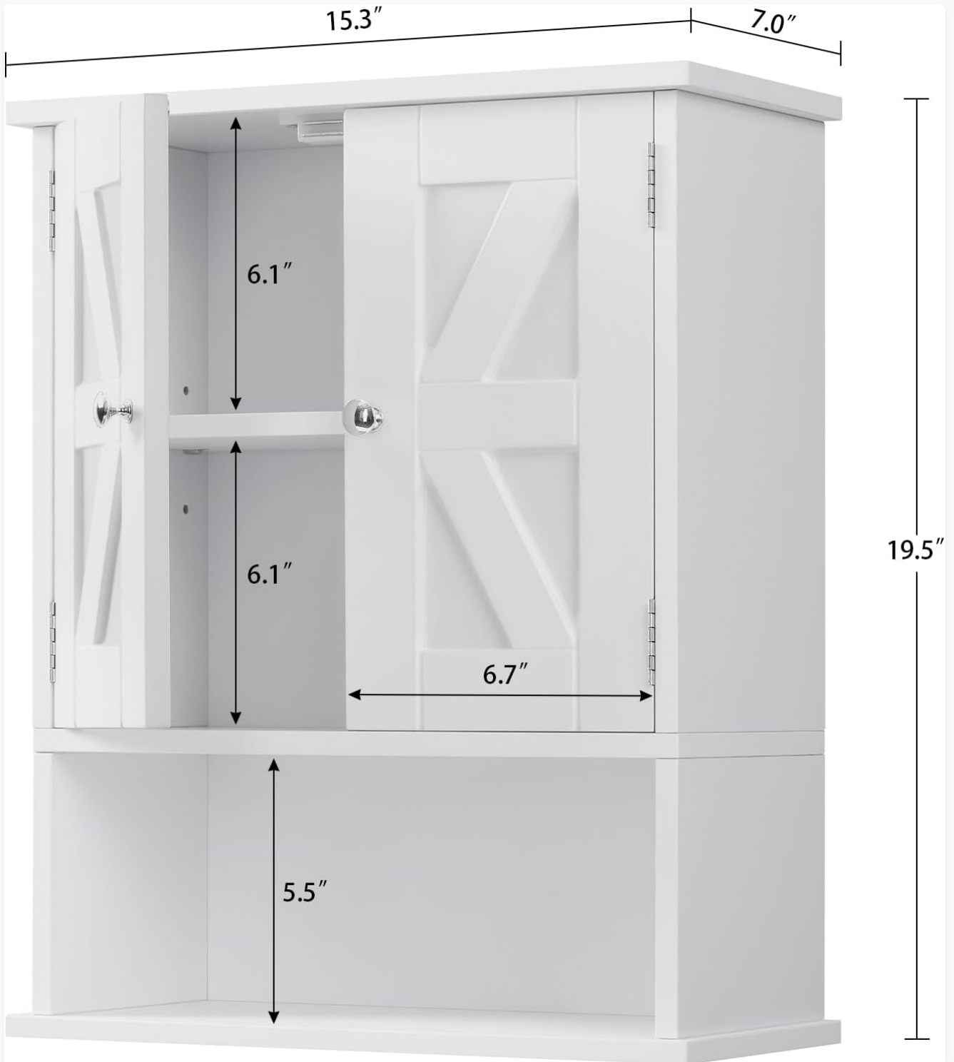
Detailed dimensions of the cabinet, including internal shelf spacing and overall size.
