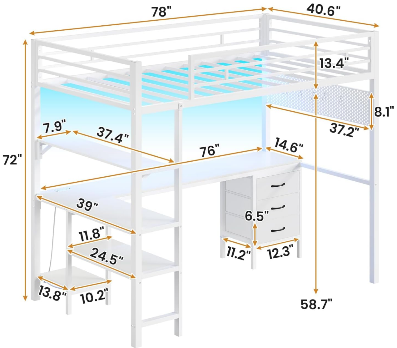
Image 8.1: Product dimensions overview.
