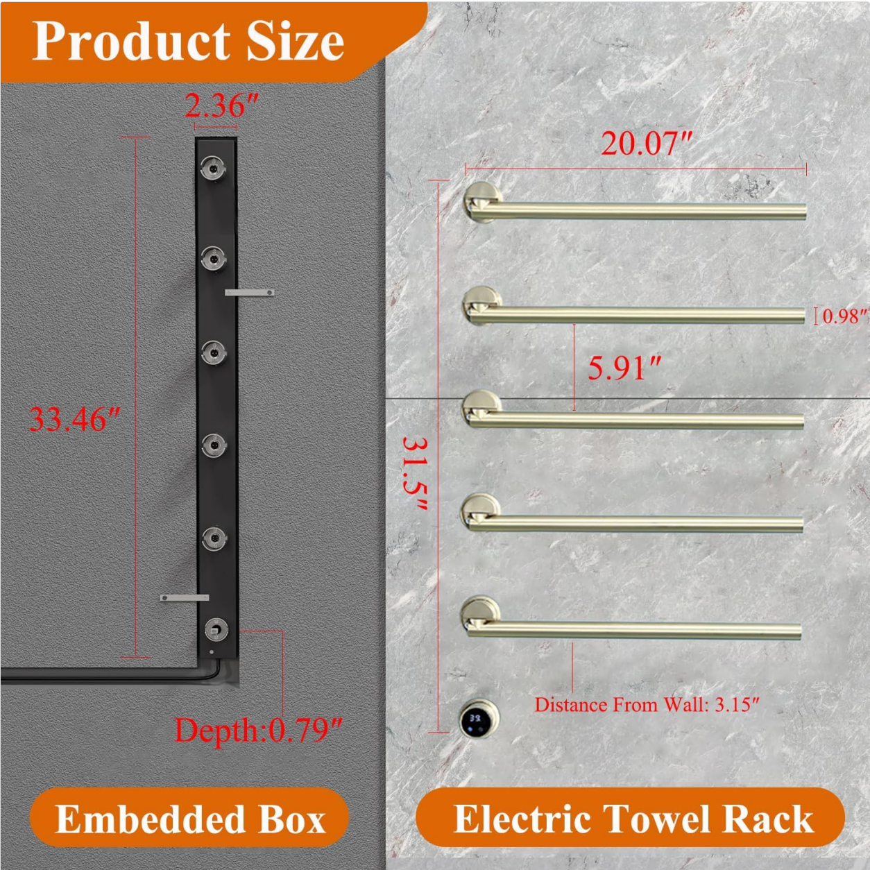
Image: Detailed product dimensions for both the embedded box and the visible electric towel rack.
