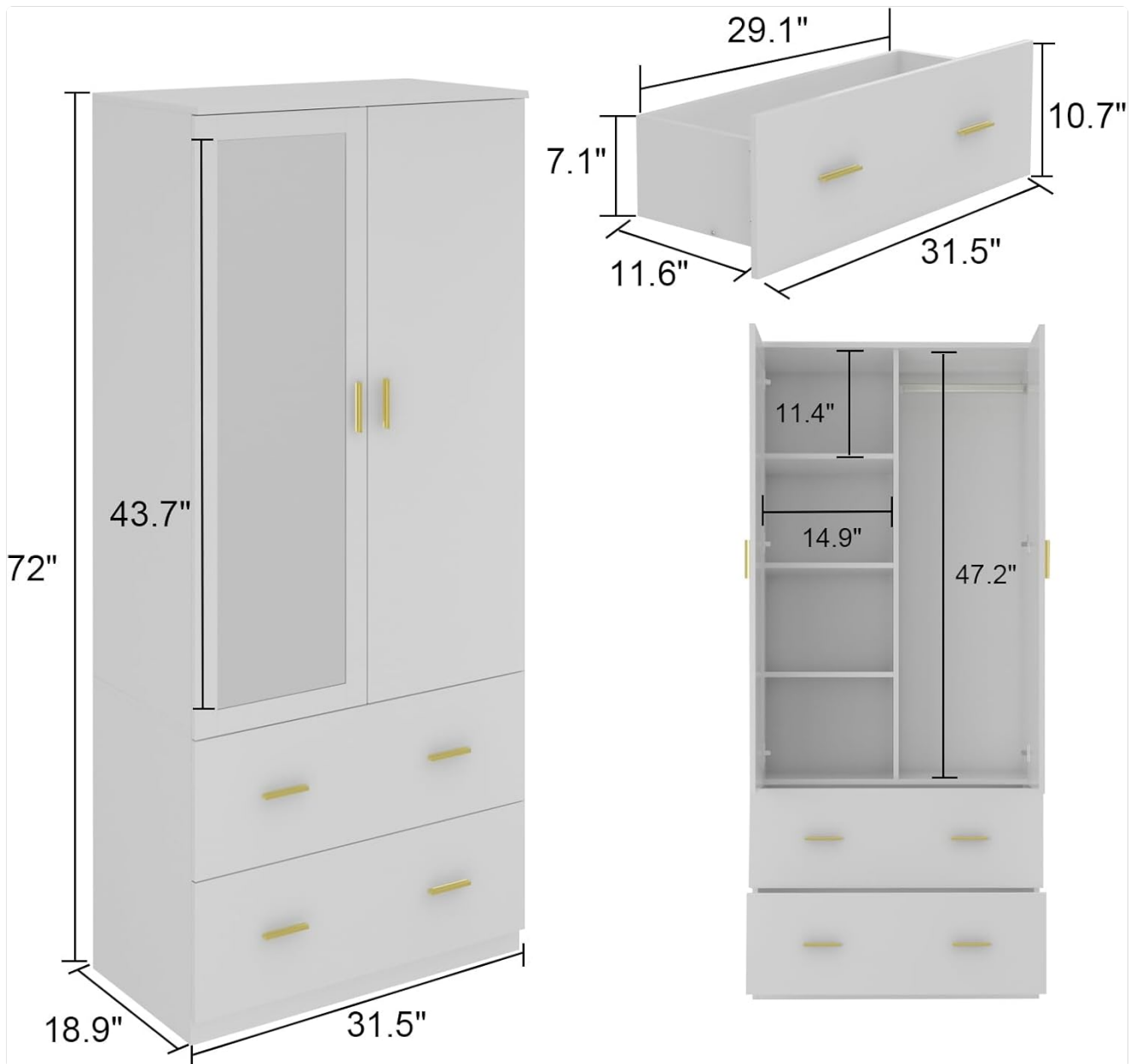
Image: Comprehensive dimension diagram for the Hitow 2 Door Wardrobe Armoire.
