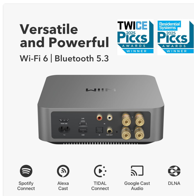
Figure 3.2: Rear view of the WiiM Amp Pro, detailing all available input and output ports for connectivity.
