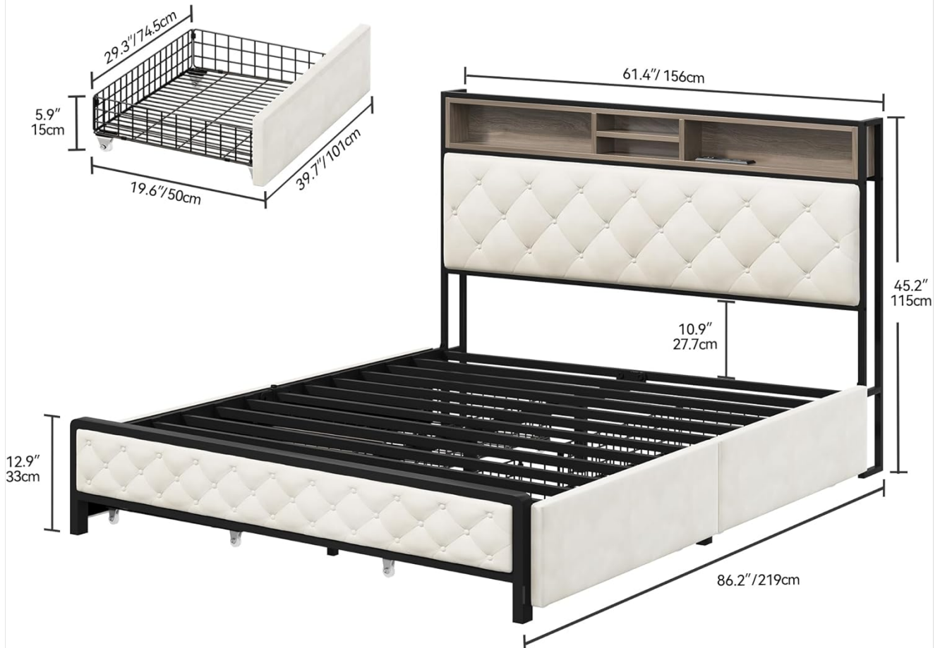
Image 2.1: Detailed diagram showing the dimensions of the bed frame and the 1100 lbs weight capacity.
