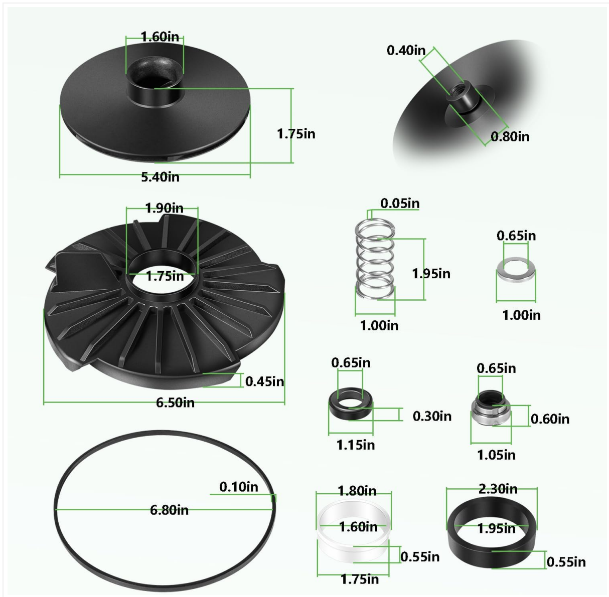
Figure 8: Detailed dimensions for the impeller, diffuser, and seal components.
