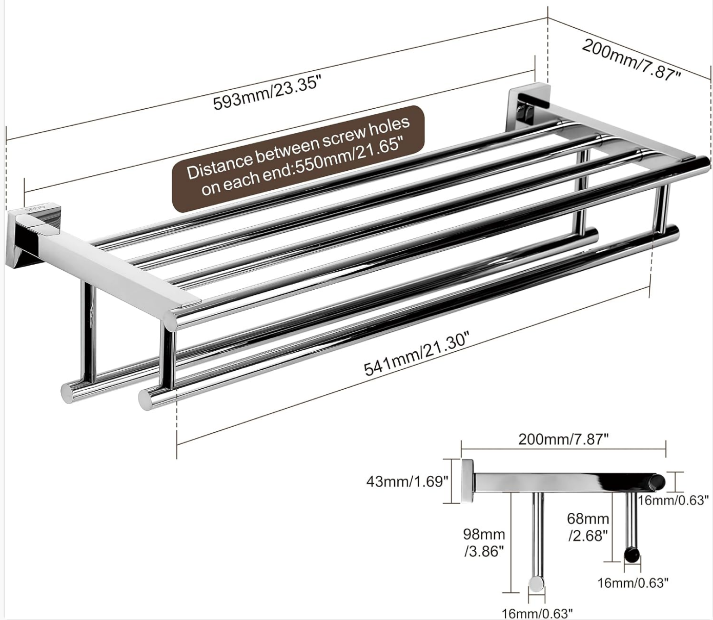
Figure 4: Detailed reference dimensions for the SEIDO Double Towel Rack.
