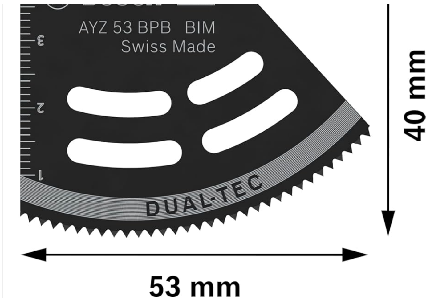
Image 7.1: The AYZ 53 BPB blade illustrating its key dimensions: 53 mm width and 40 mm cutting depth.
