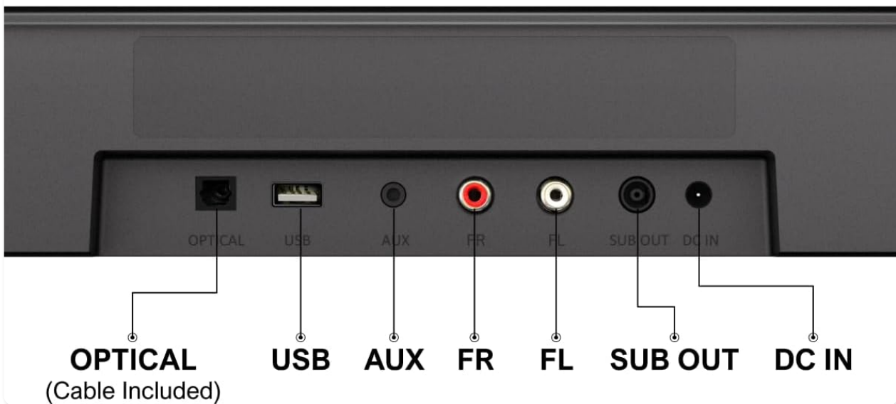
Figure 2: Included components of the ULTIMEA Aura A40 system.
