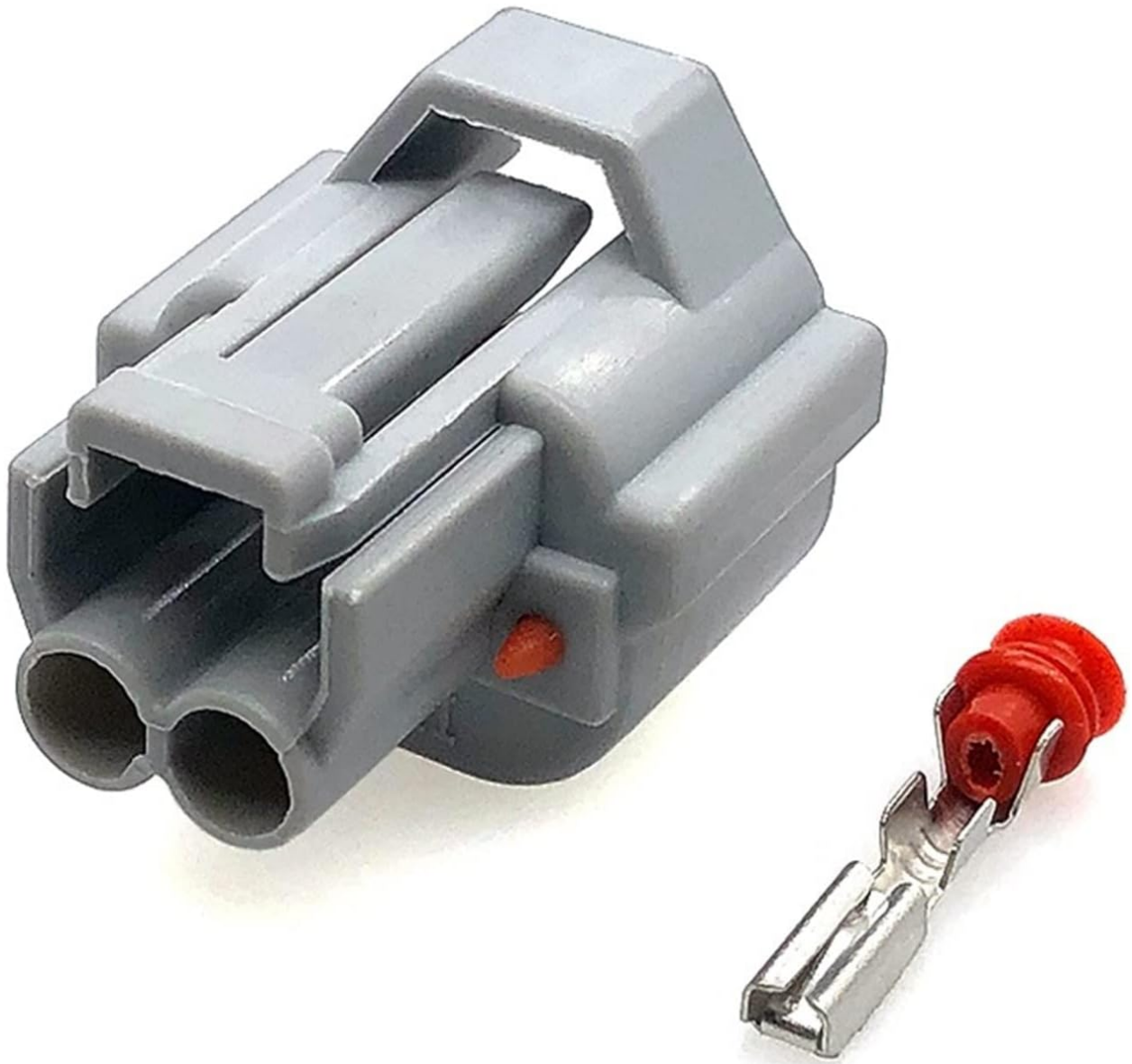
Figure 3.3: Rear view of the connector housing, showing the wire entry points. This view illustrates where the wires, once crimped to the terminals, will enter the connector body.
