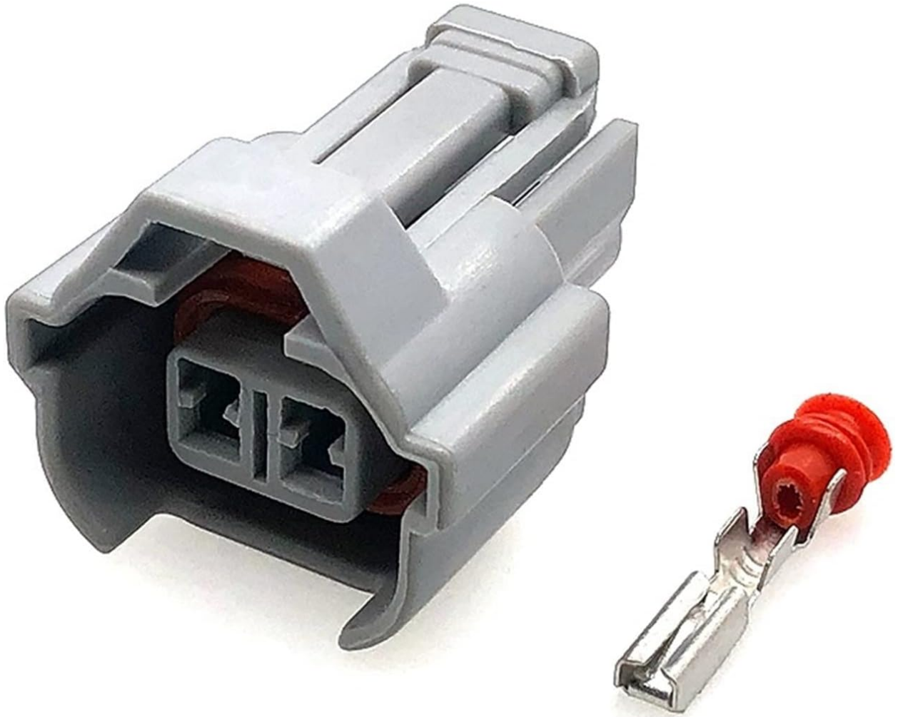
Figure 3.1: Front view of the 2-pin connector housing with a terminal and red seal. This image shows the main connector body and one of the metal terminals with its red waterproof seal, ready for assembly.
