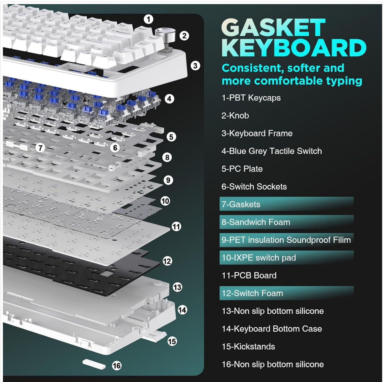
Figure 3.2: Gasket Keyboard Structure Diagram
