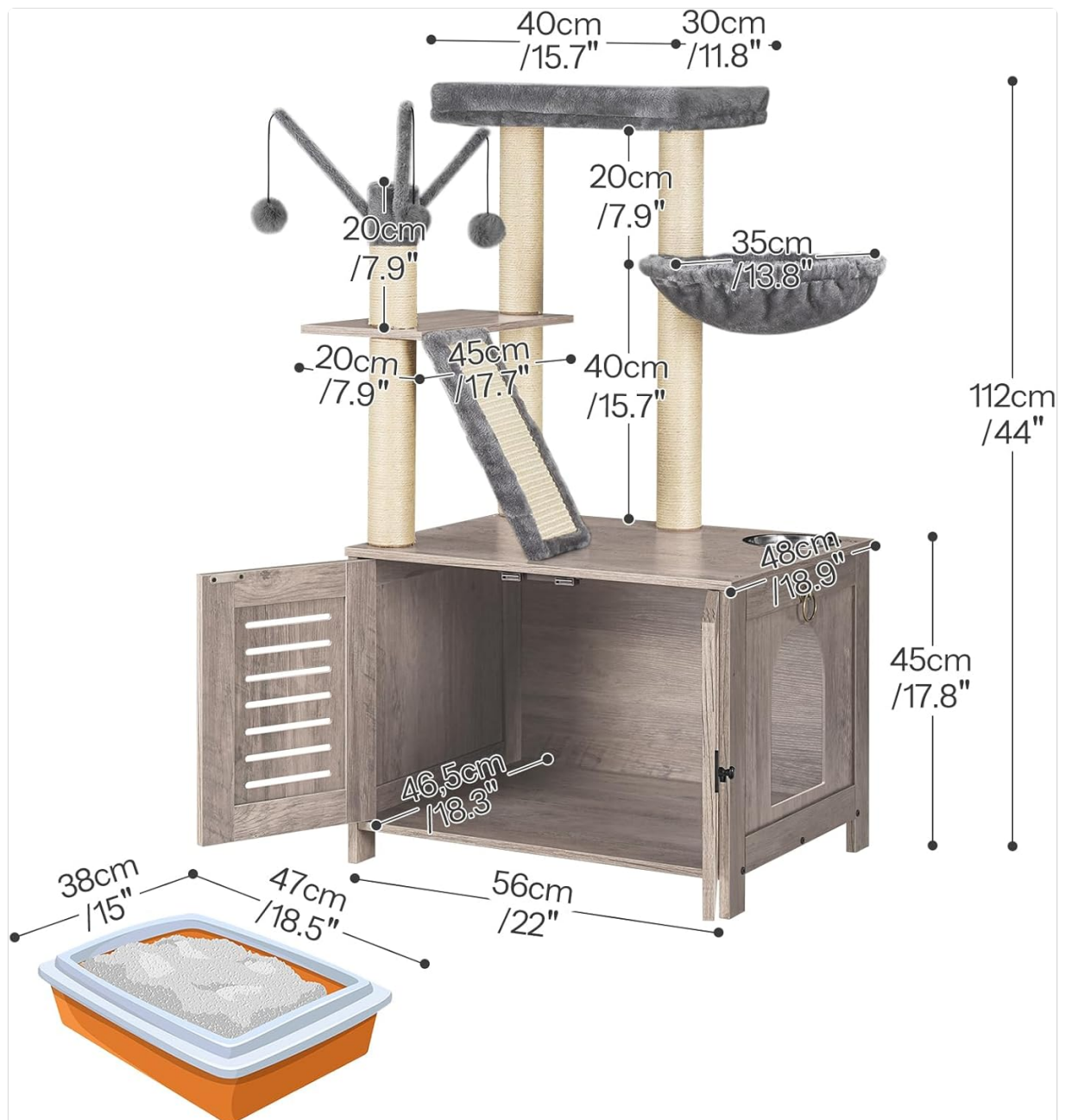
Image 8.1: Detailed dimensions of the HOOBRO BG48MZ03 Cat Tree.
