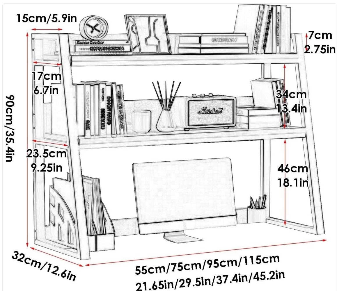
Image: Detailed dimensions of the Ktop Office Storage Rack, including shelf heights and overall measurements.
