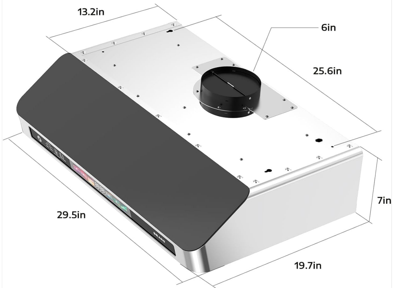
Figure 4.1: Detailed dimensions of the range hood for installation planning.
