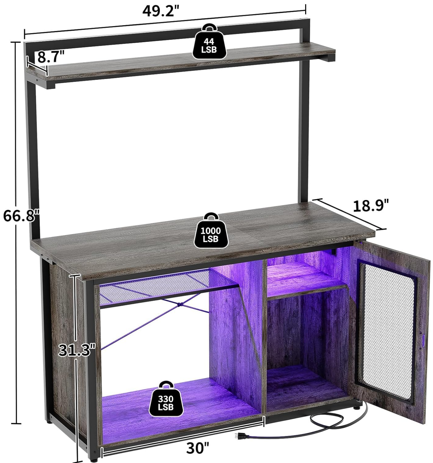
Figure 3: Dimensions and load capacities of the stand.
