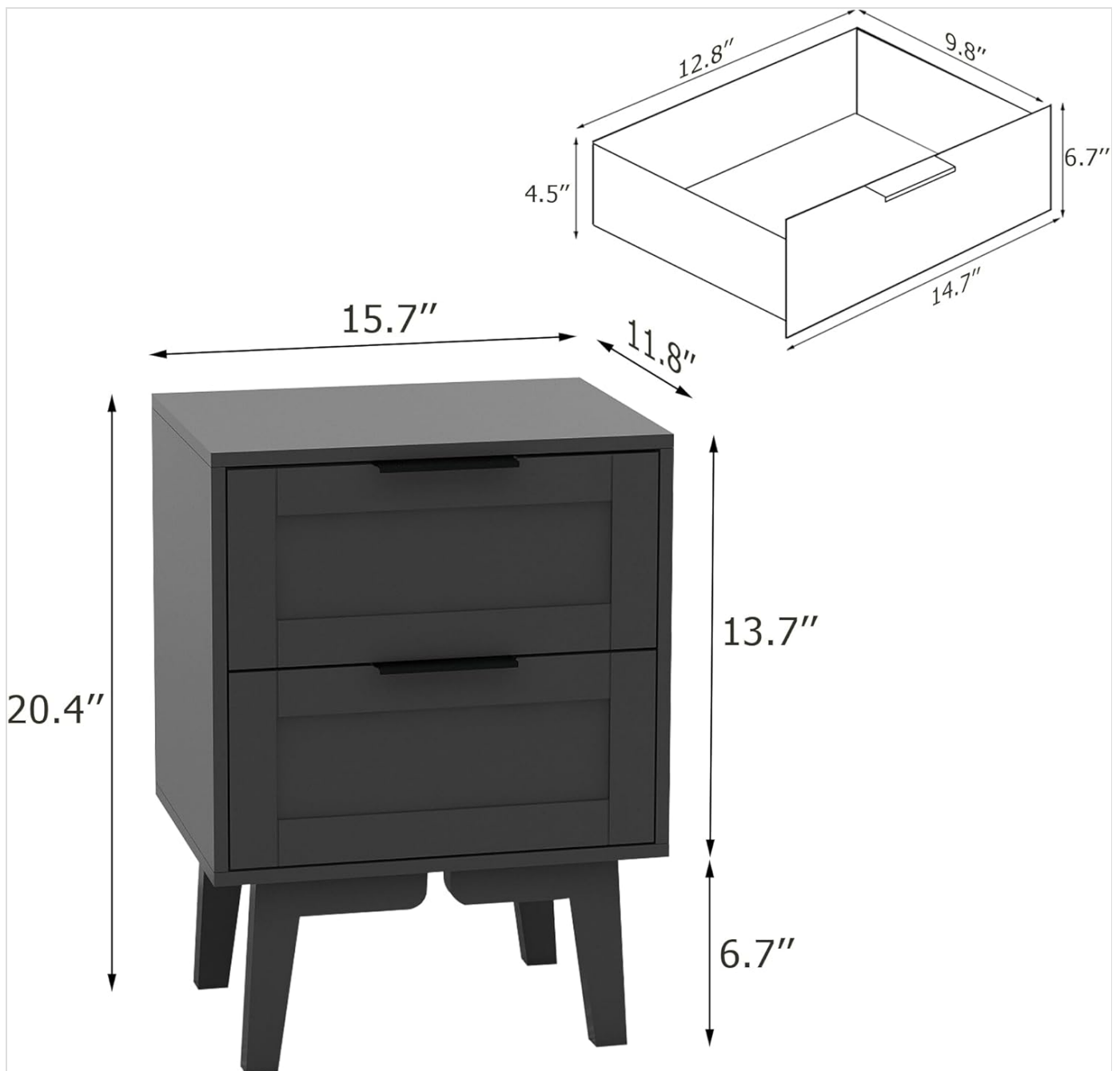
Image: Detailed dimensions of the nightstand and its drawers.
