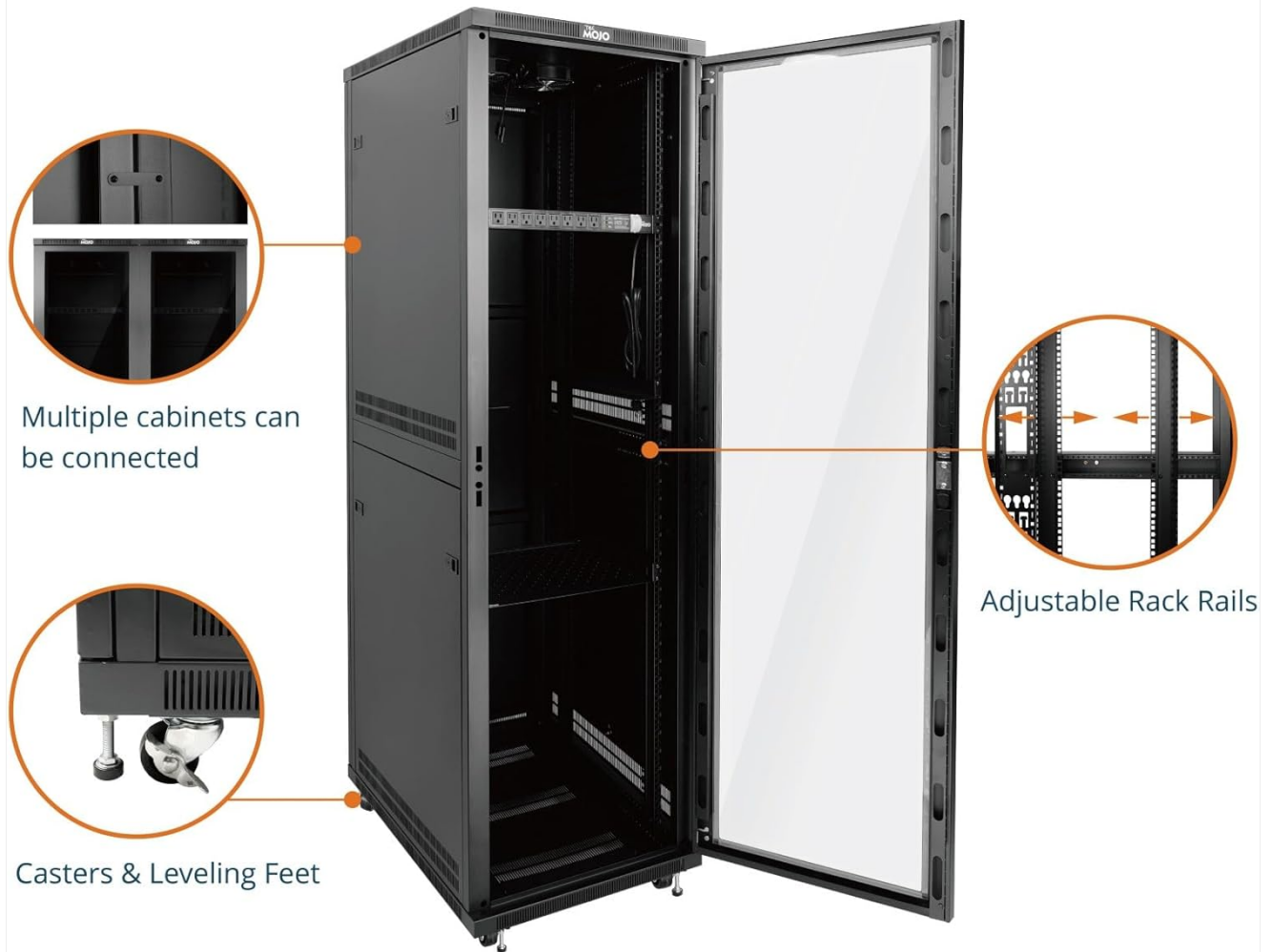
Figure 4: The Tecmojo 42U Network Cabinet includes a PDU, shelf, and cooling fans. It also features adjustable rack rails, casters, and leveling feet for flexibility and mobility.
