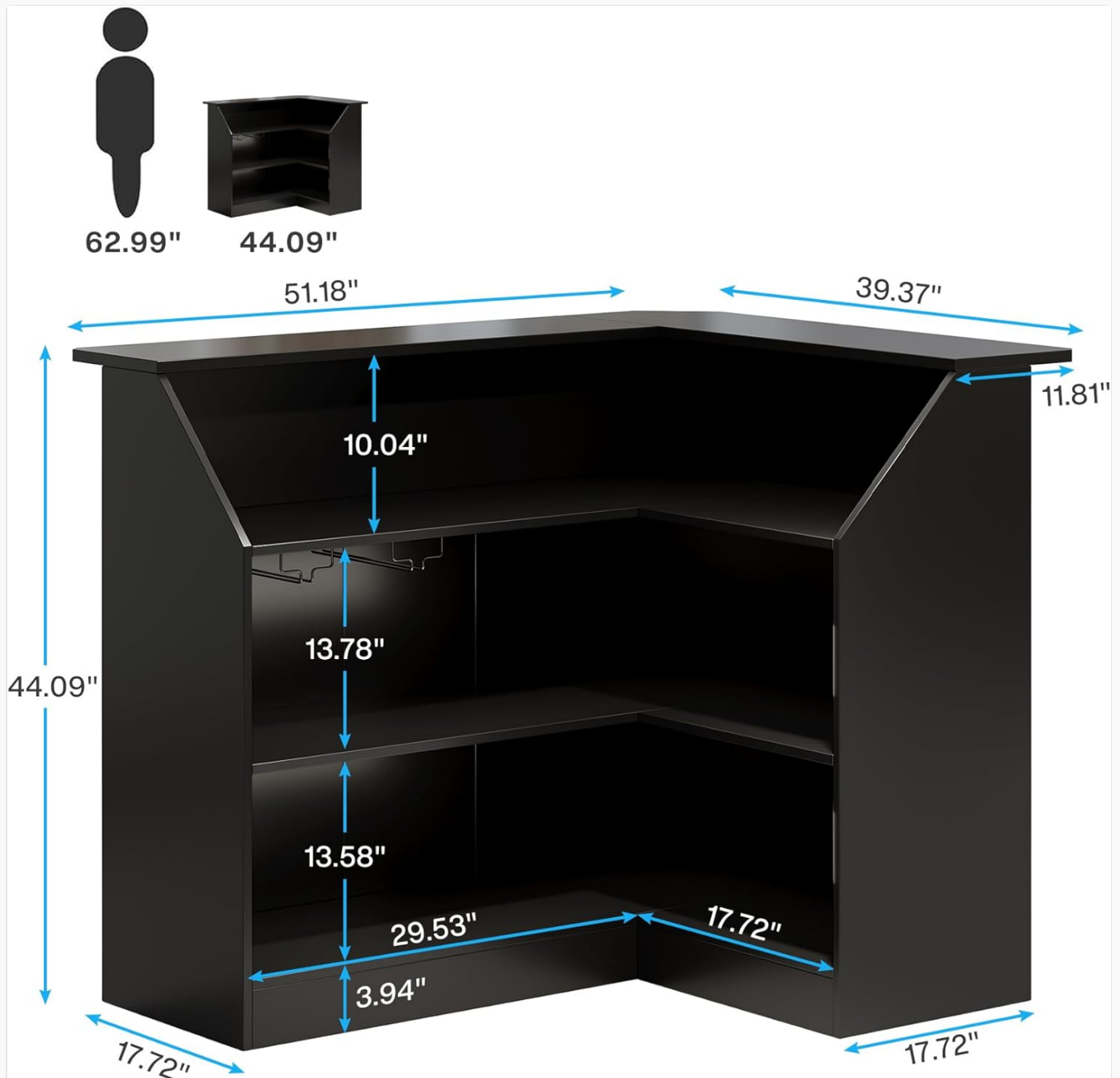
Image 2: Dimensional overview of the L-shaped bar cabinet.
