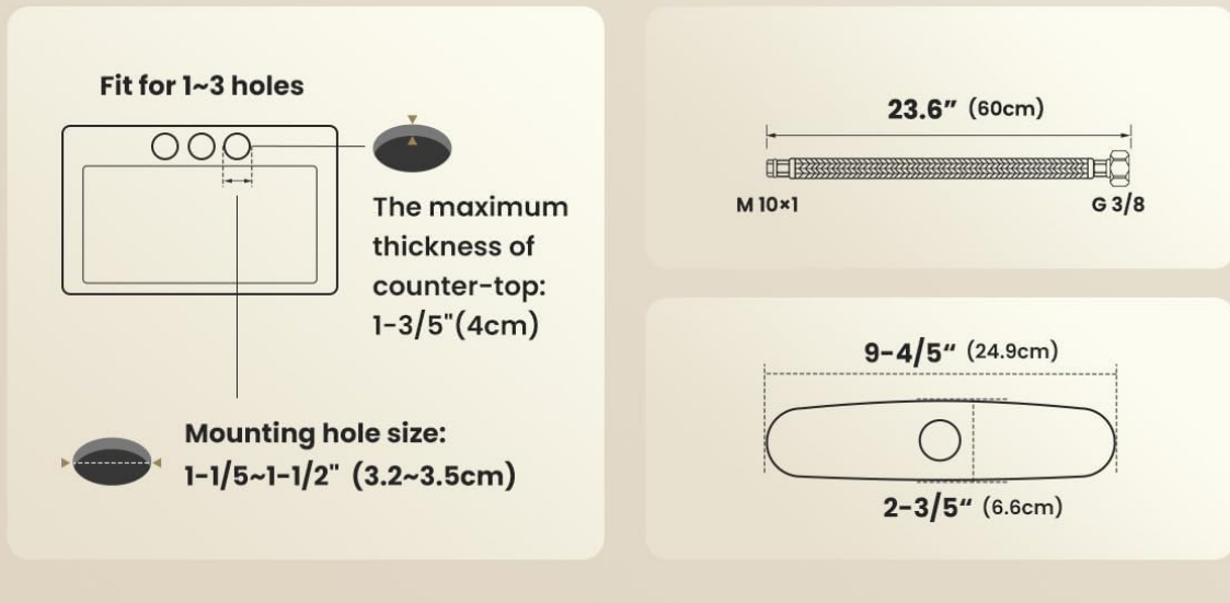
Figure 3: Faucet Dimensions and Mounting Requirements
