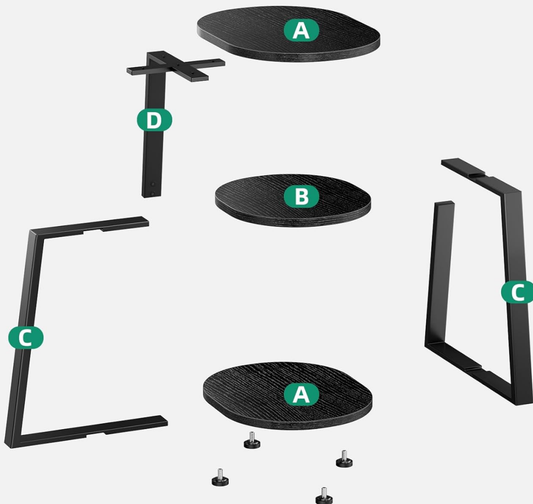
Image: Exploded view of the Kalrin Side Table components, showing shelves, frame pieces, and hardware.
