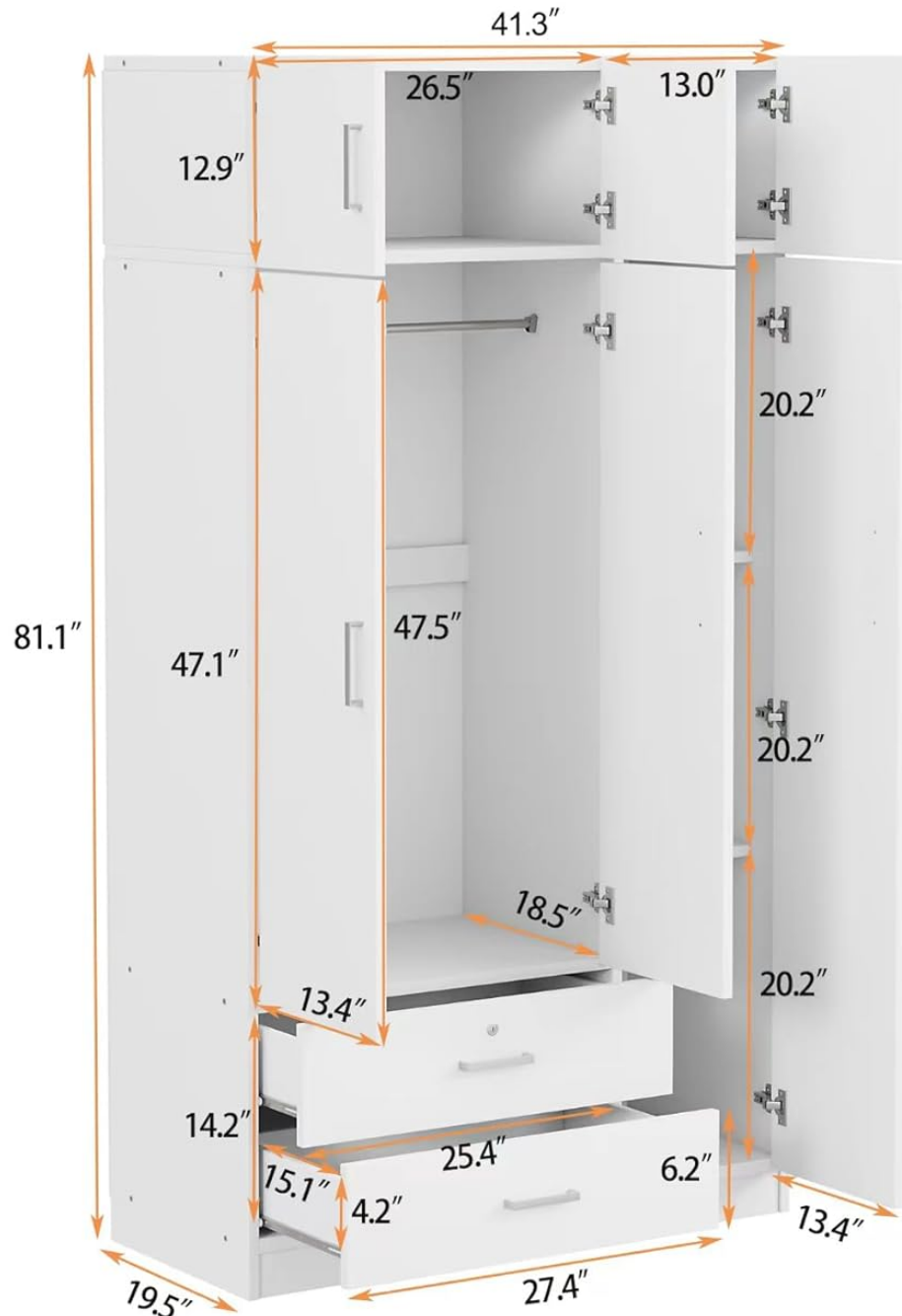
Figure 4.1: Detailed dimensions of the wardrobe.
