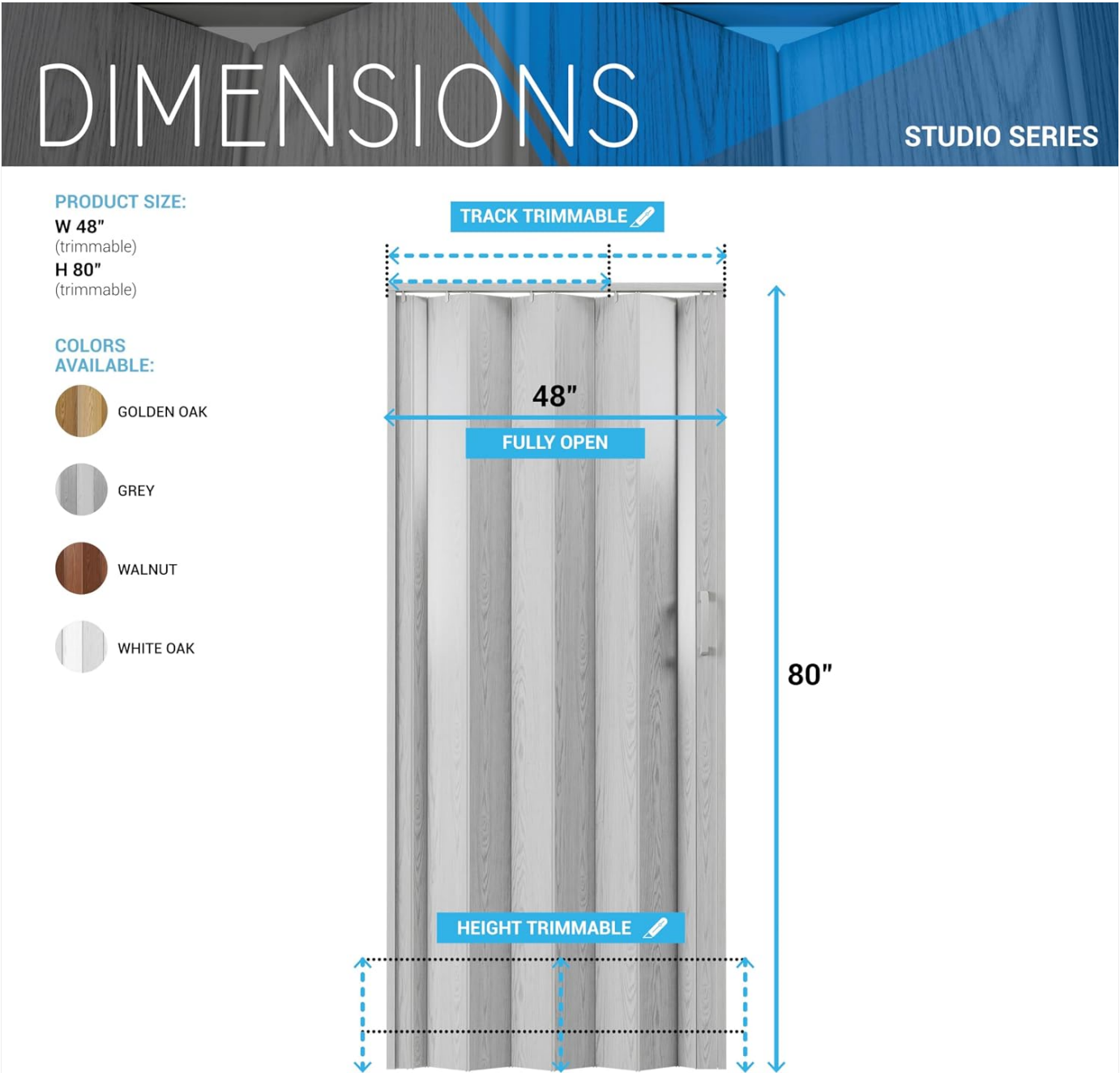
Figure 2: Trimmable dimensions for custom fitting, showing the 48-inch width and 80-inch height, and indicating where trimming can occur.
