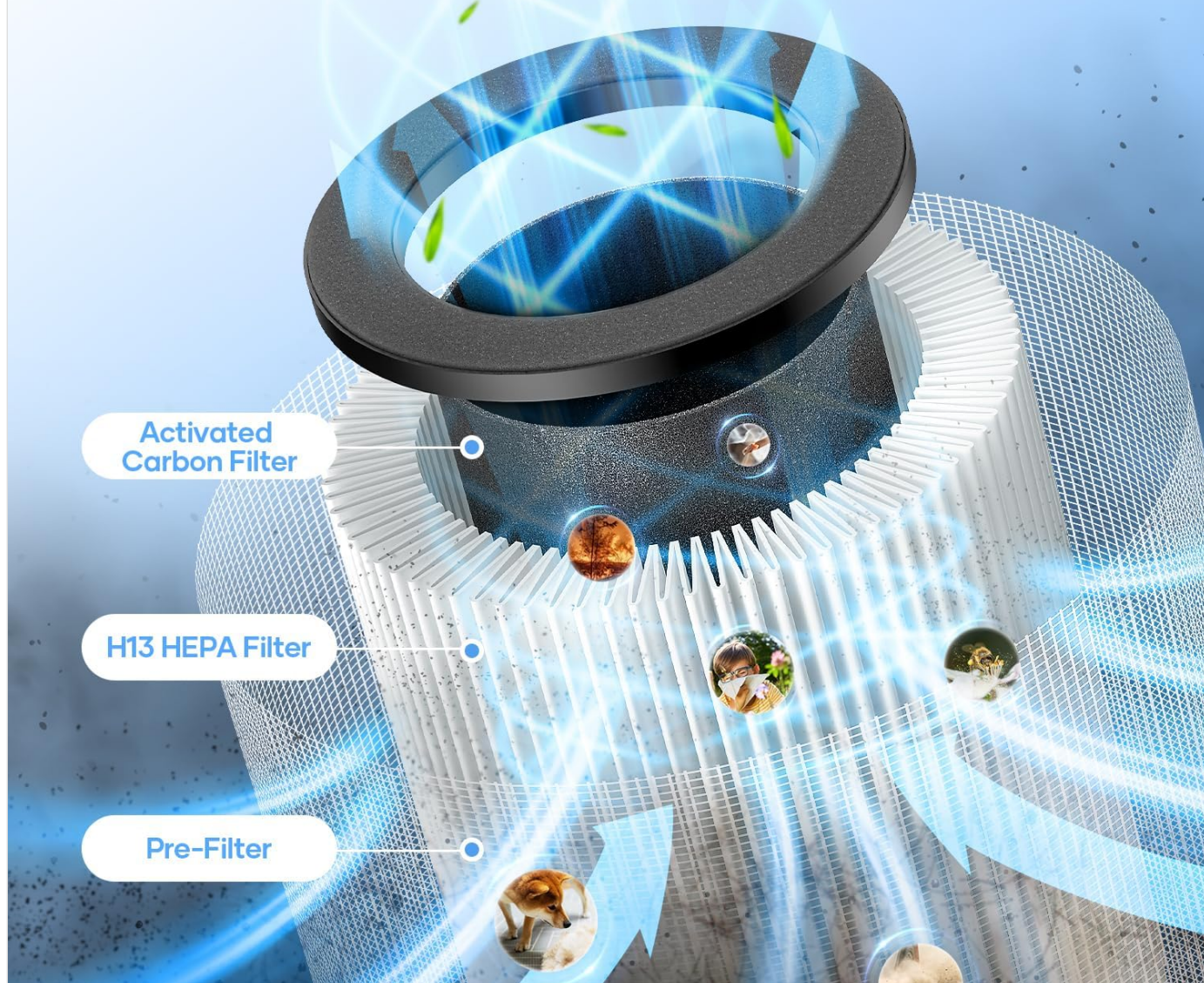
Image: A cutaway diagram illustrating the three layers of the filter: Pre-Filter, H13 HEPA Filter, and Activated Carbon Filter, showing how air passes through them to remove various pollutants.
