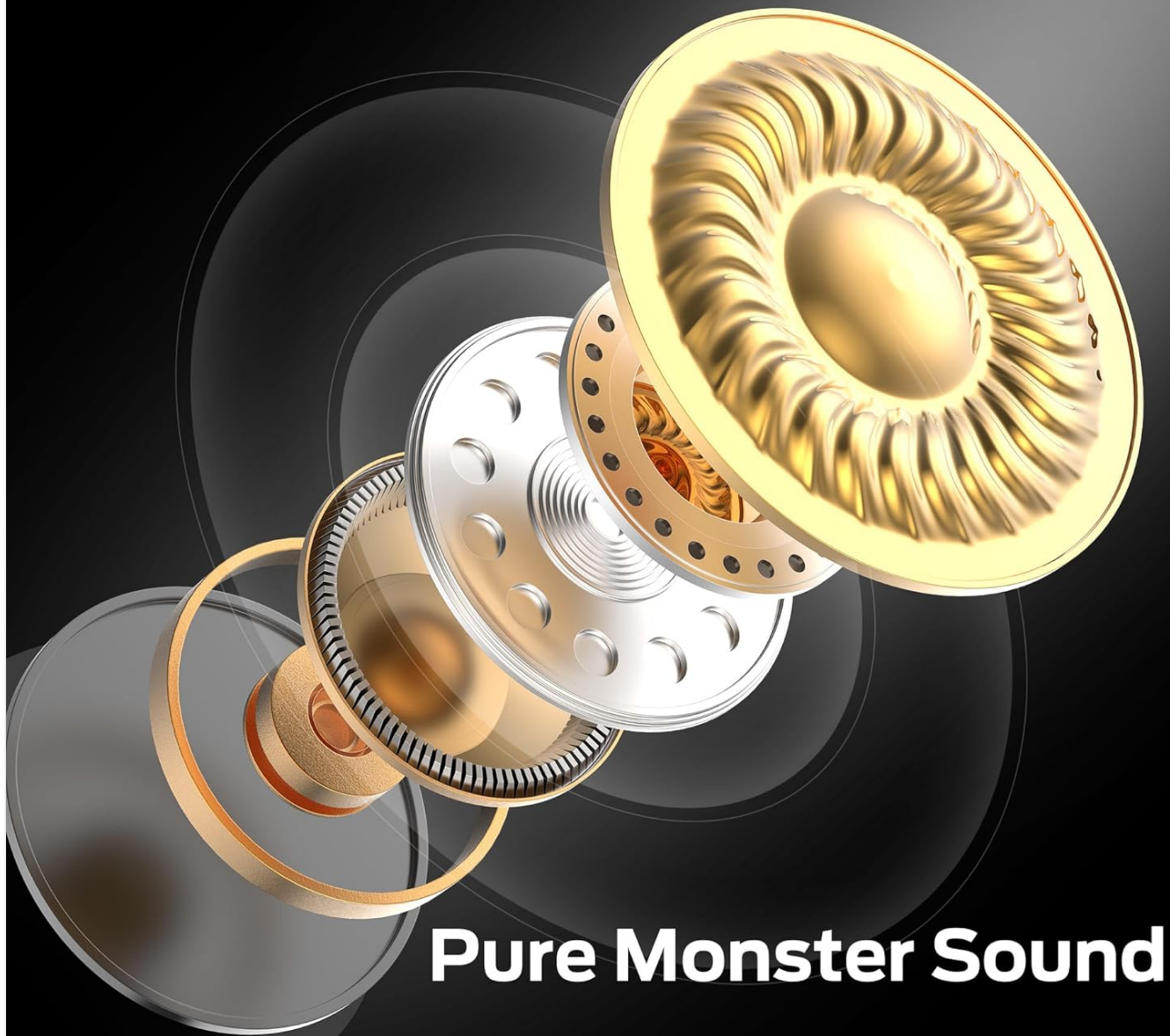
Figure 2: Exploded view illustrating the internal components of a Monster N-Lite 208 earbud driver, highlighting the layers that contribute to the "Pure Monster Sound."
