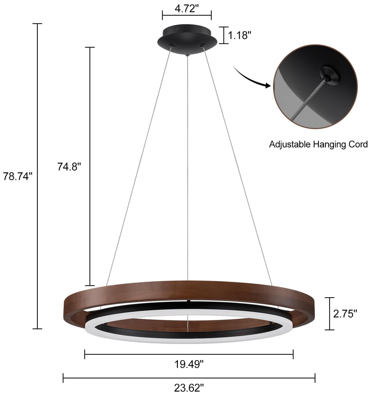
Image 4.2: This diagram illustrates the dimensions of the chandelier, including the 23.62-inch diameter, 2.75-inch height, and adjustable hanging cord up to 78.74 inches.
