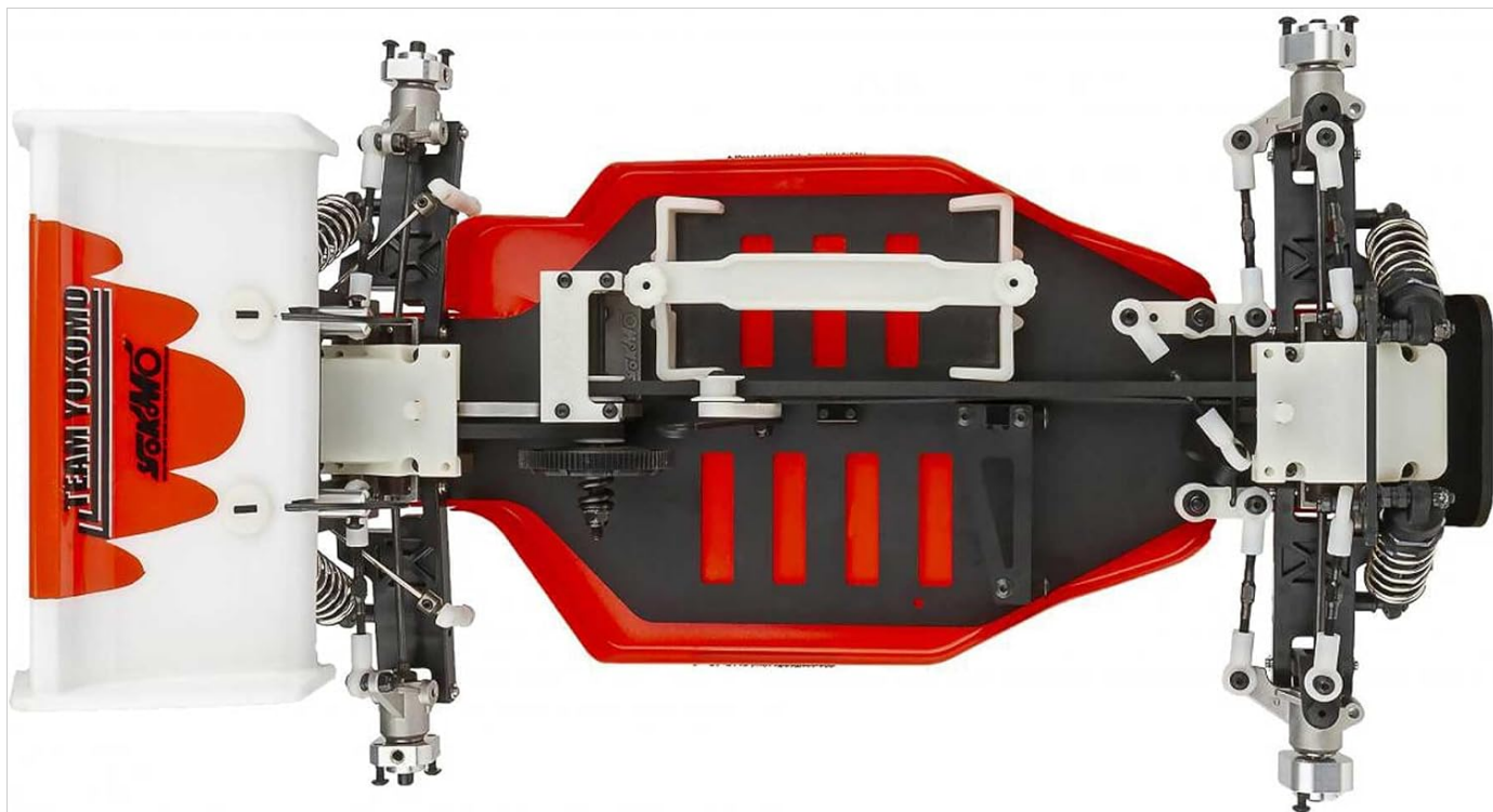
Image 2.2: Top-down view of the YZ-10 chassis, highlighting the layout of the belt drive system and component mounting points.
