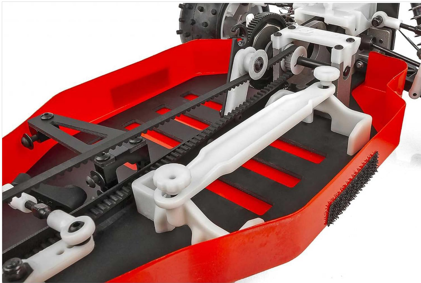
Image 4.2: Detailed view of the chassis and belt drive system, showing areas where debris can accumulate and require cleaning.
