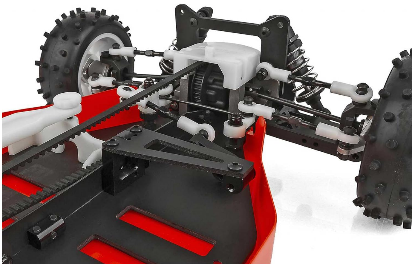
Image 2.3: Close-up of the 4WD belt drive system, showing the belts, pulleys, and gear arrangement.
