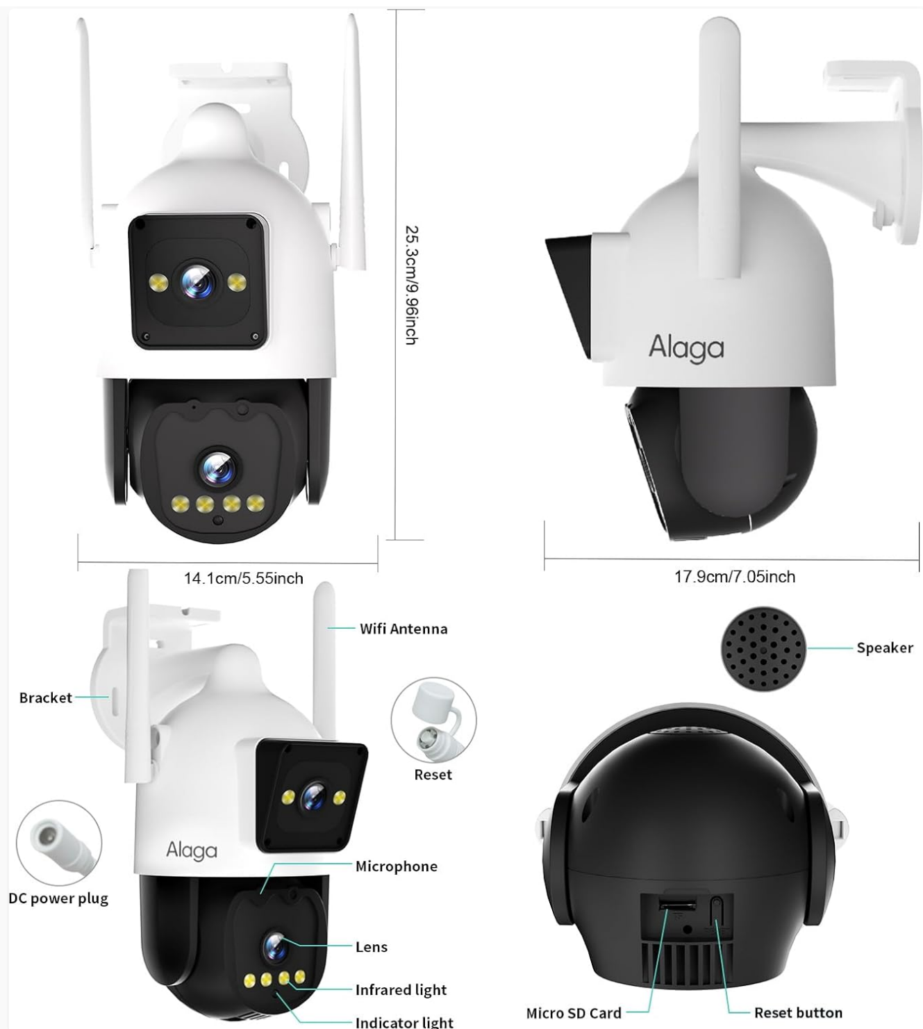
Figure 2.1: Detailed diagram of the Alaga Outdoor Security Camera showing its dimensions and key components such as Wi-Fi antennas, lenses, microphone, speaker, DC power plug, and Micro SD card slot.
