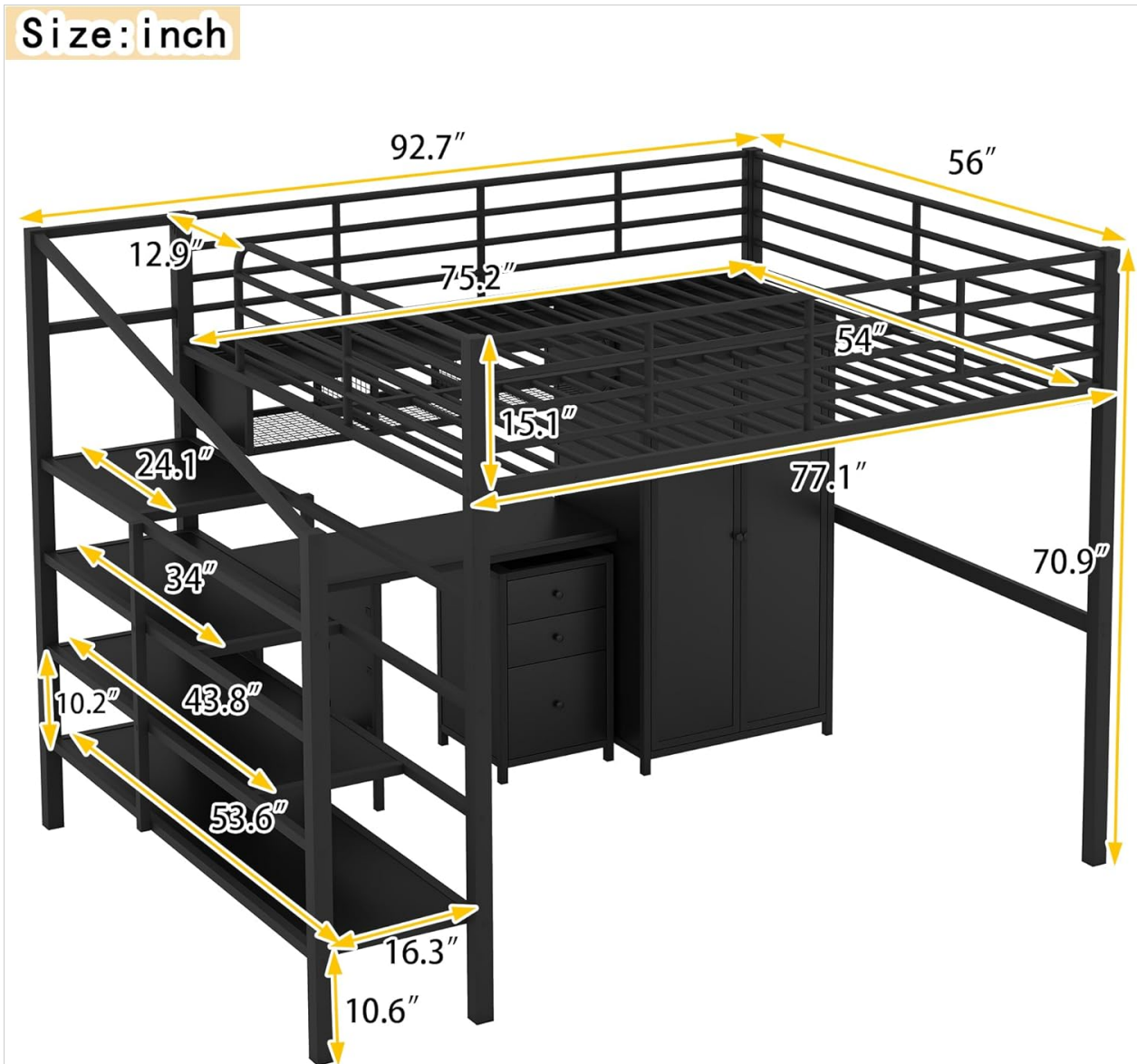
Image 2: Dimensional diagram of the loft bed.
