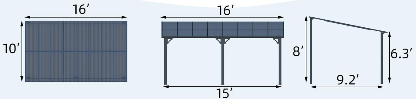
Figure 8.1: Detailed dimensions of the AECOJOY 16' x 10' Hardtop Gazebo.
