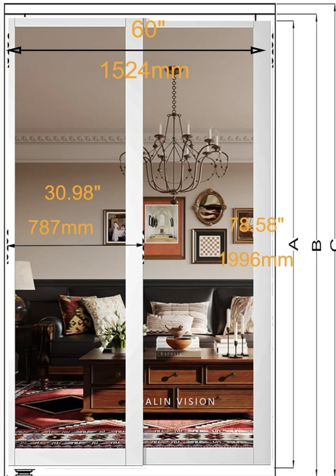
Image 4.1: Refer to the size chart to ensure compatibility with your door opening. Note the actual panel dimensions versus the recommended opening size.
