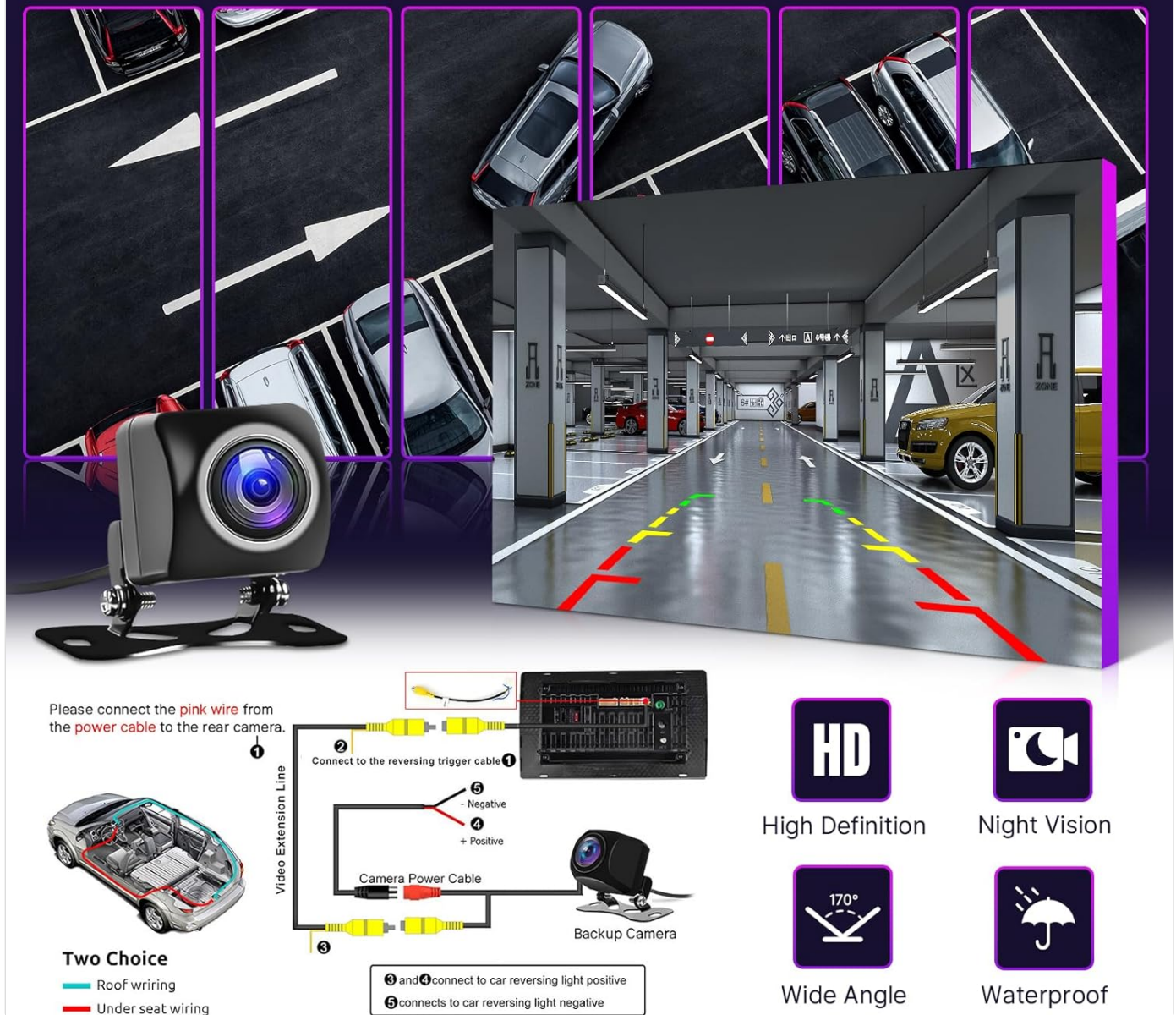
Figure 3.2: Backup camera wiring diagram and display example.
