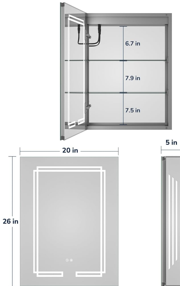
Image: Dimensions of the Keonjinn 20x26 Inch LED Medicine Cabinet, showing external measurements and internal shelf spacing.
