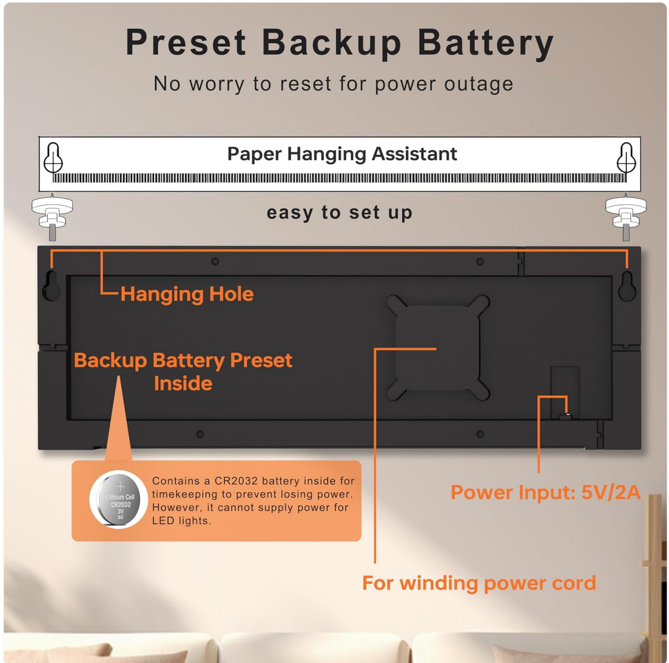
Image: Rear view of the JALL digital clock, highlighting the power input (5V/2A) and the internal CR2032 backup battery compartment. The backup battery is for timekeeping memory during power outages, not for powering the display.
