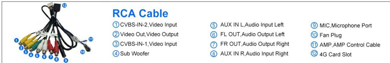
Figure 3: Wiring diagram for single climate control and RCA cable connections.
