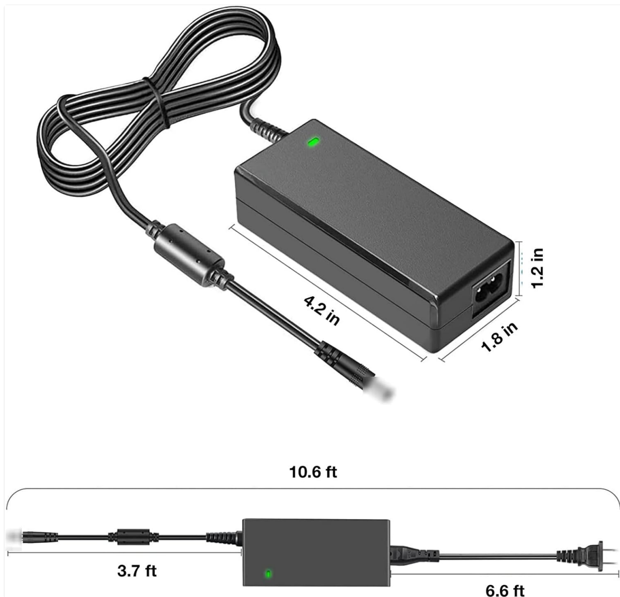
Figure 1: AC Adapter with key dimensions. The adapter unit measures approximately 4.2 inches in length, 1.8 inches in width, and 1.2 inches in height. The total cable length is approximately 10.6 feet, with the DC output cable being 3.7 feet and the AC input cable being 6.6 feet.
