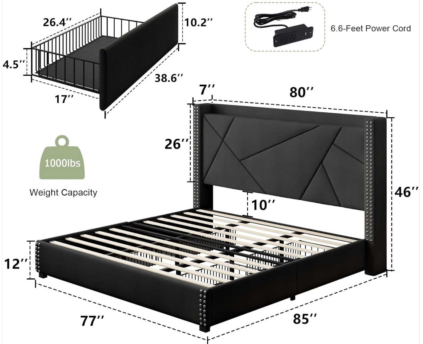
Figure 4.3: The Feonase bed frame with all four storage drawers extended.
