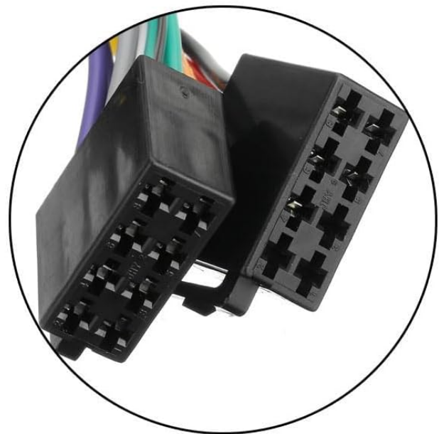
Figure 4.1: Diagram illustrating the ISO wiring harness connections, showing the male and female connector types and their pin configurations for power and signal.
