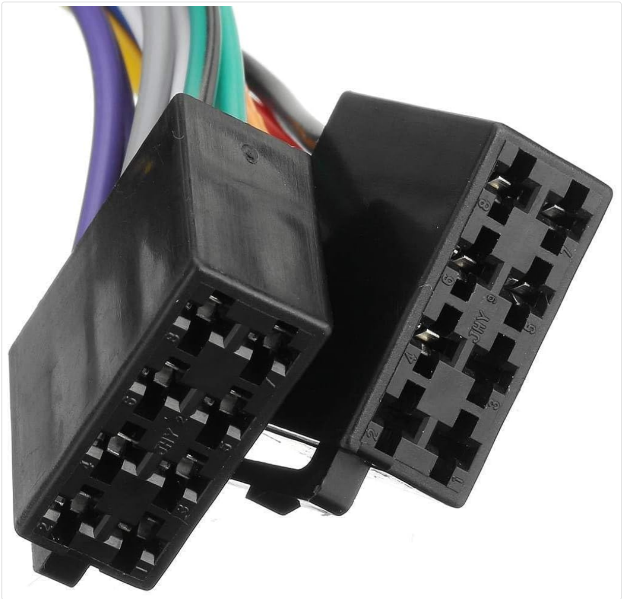
Figure 4.2: A close-up view of the male connector pins, showing the precise arrangement for secure electrical contact.
