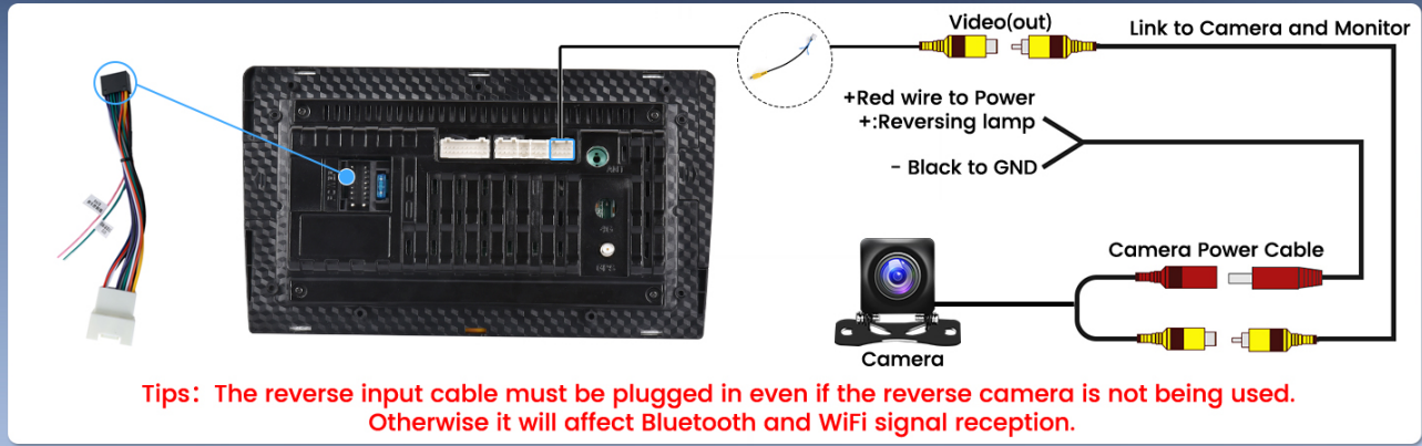
Image: Detailed wiring diagram for the backup camera connection, showing connections to the car stereo, power, and reversing lamp.
