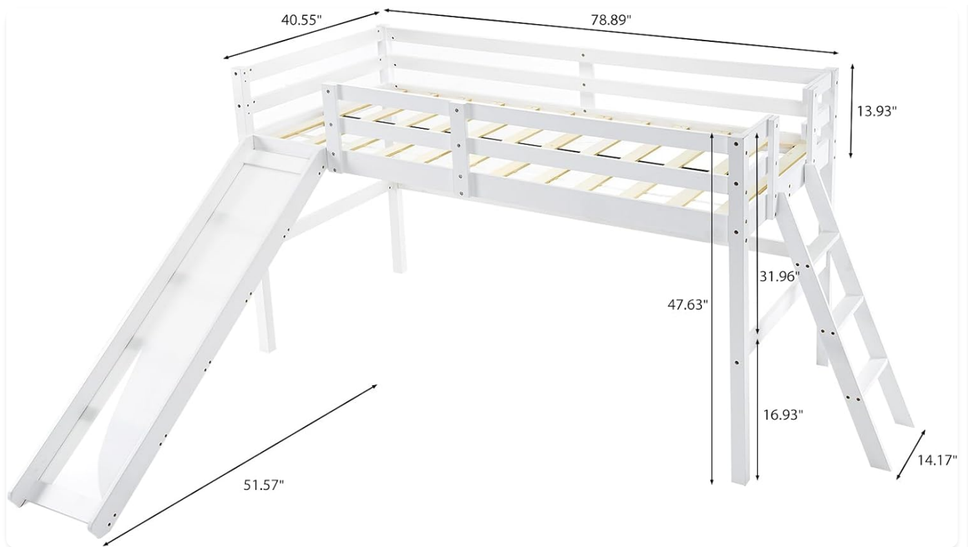
Image 1.2: Detailed dimensions of the VINGLI Twin-Slide Loft Bed, including length, width, and height measurements for the bed frame, slide, and ladder.
