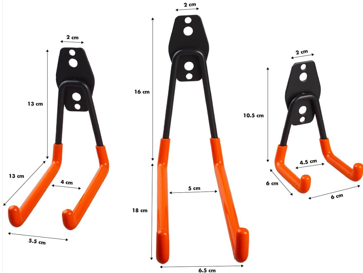
Image 6.1: Dimensional comparison of Maclean hook models MC-443, MC-444, and MC-442. The MC-443 measures approximately 13 cm in height and 13 cm in arm length, with a 5.5 cm width between arms.
