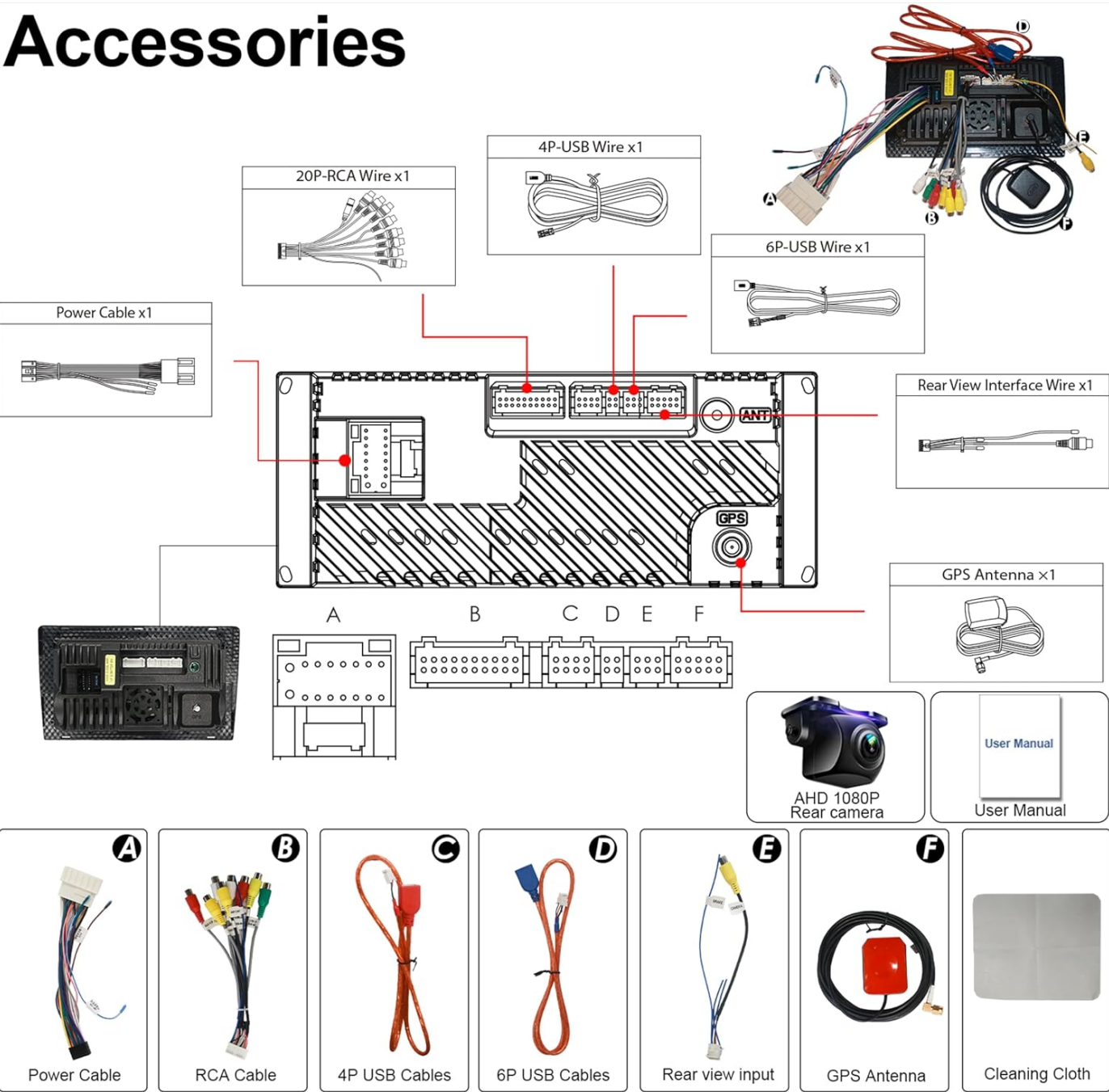
Image 3.1: Detailed view of all cables and accessories included with the car radio, along with a wiring diagram for connection points.
