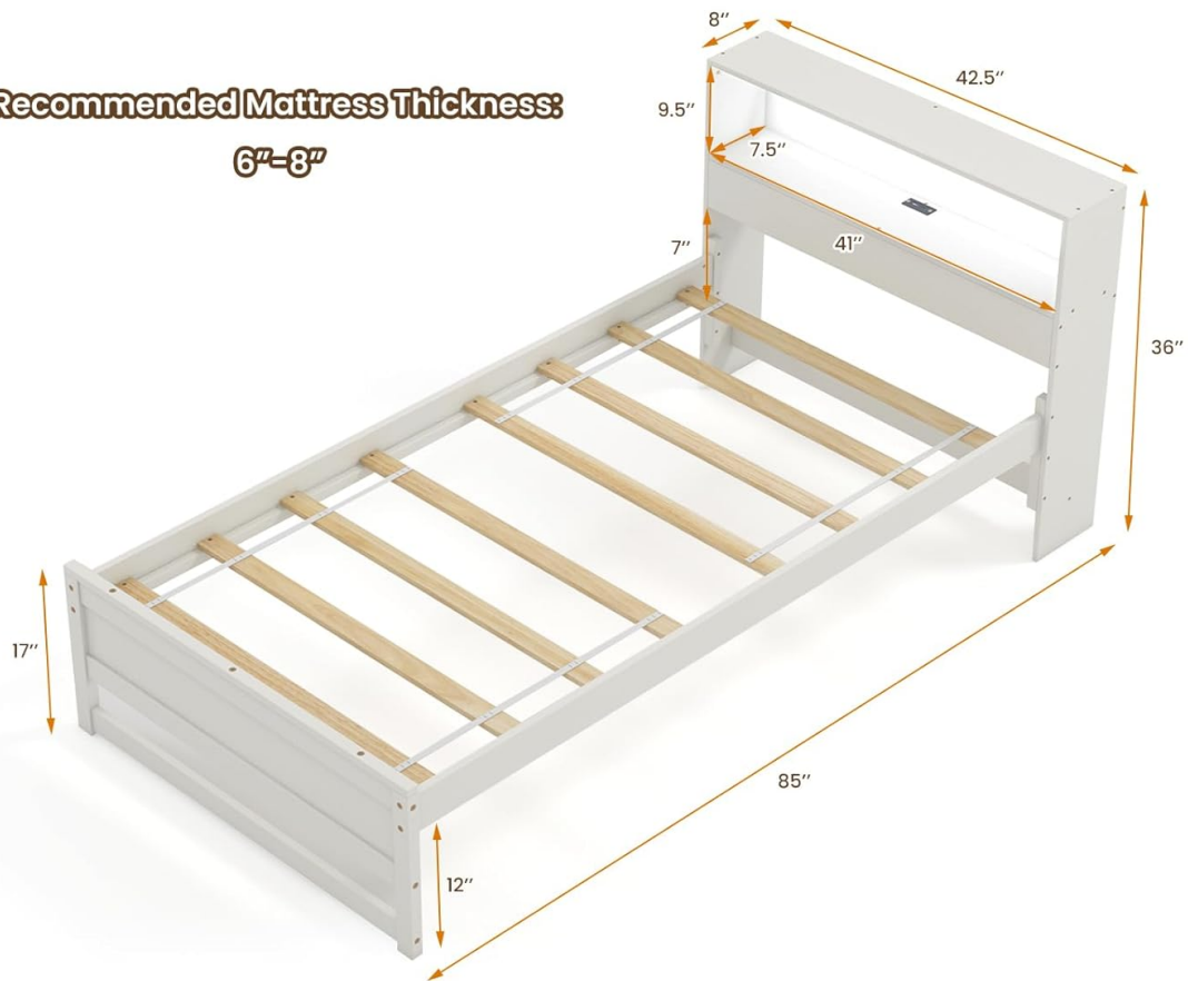
Figure 1: Overall dimensions and components of the bed frame. Note the 12-inch under-bed clearance and recommended mattress thickness of 6-8 inches.
