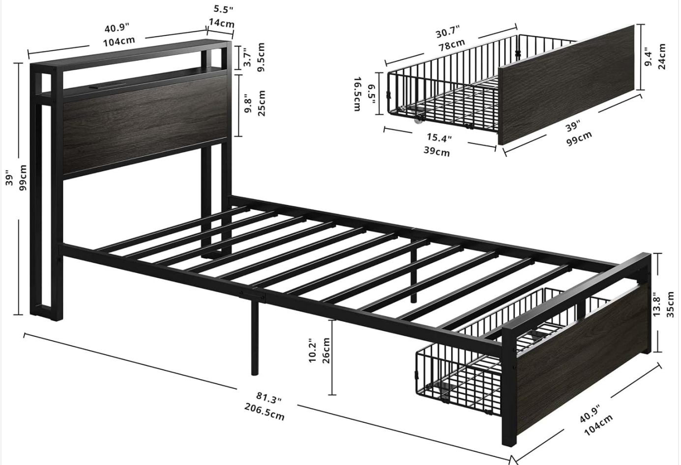
Figure 1: Exploded view of the LIKIMIO Twin Bed Frame showing all major components and dimensions. Note the integrated charging station on the headboard and the pull-out storage drawer at the foot of the bed.
