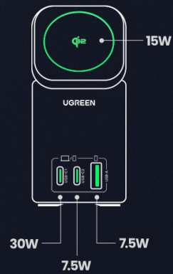
Image: Diagram illustrating power distribution when a single device is connected to the wireless pad (15W), USB-C1 (30W), USB-C2 (7.5W), or USB-A (7.5W).
