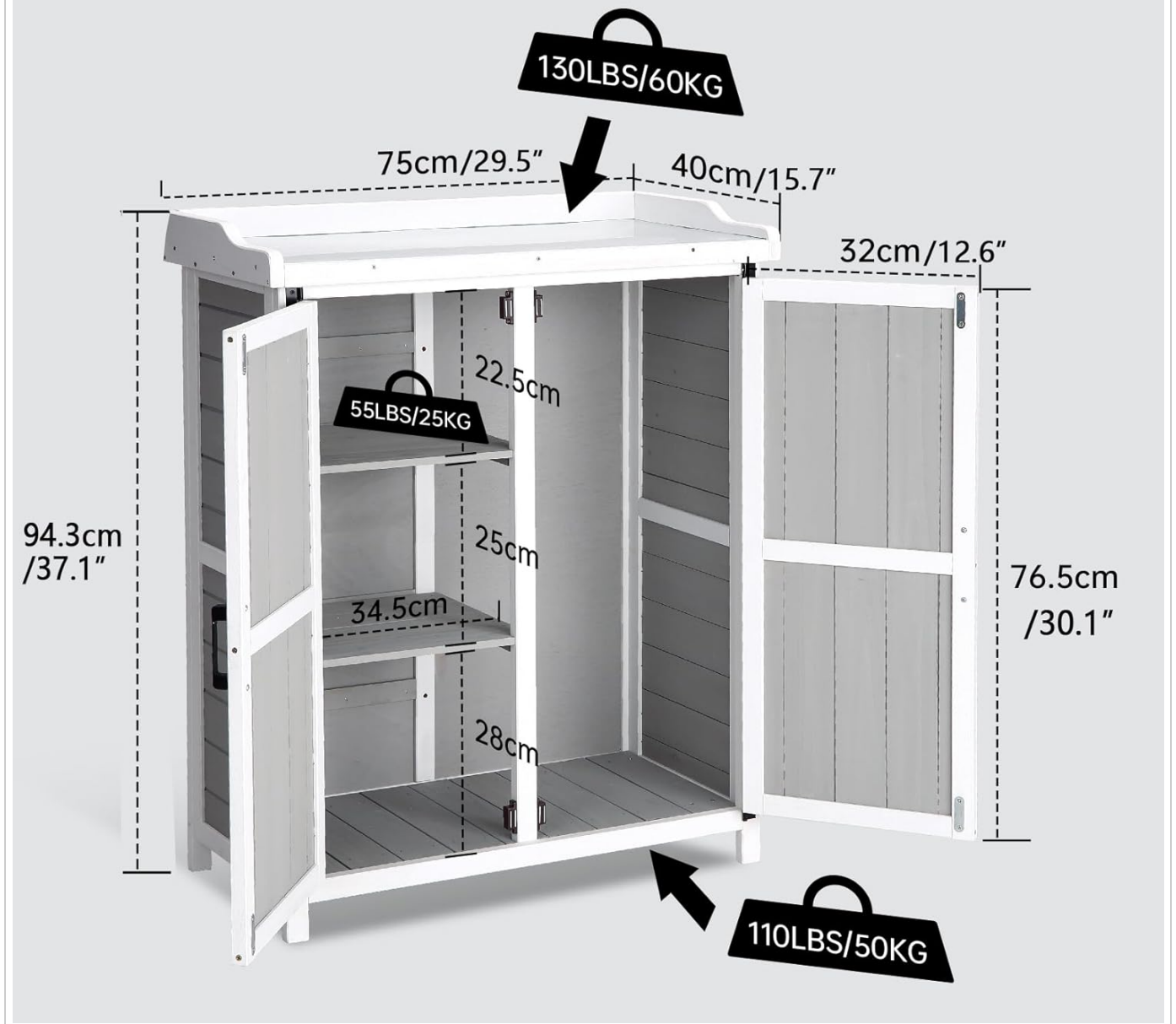
Image: Diagram illustrating the product dimensions (29.5" L x 15.7" W x 37.1" H) and load capacities: 130 lbs (60 kg) for the tabletop, 55 lbs (25 kg) per adjustable shelf, and 110 lbs (50 kg) for the bottom shelf.
