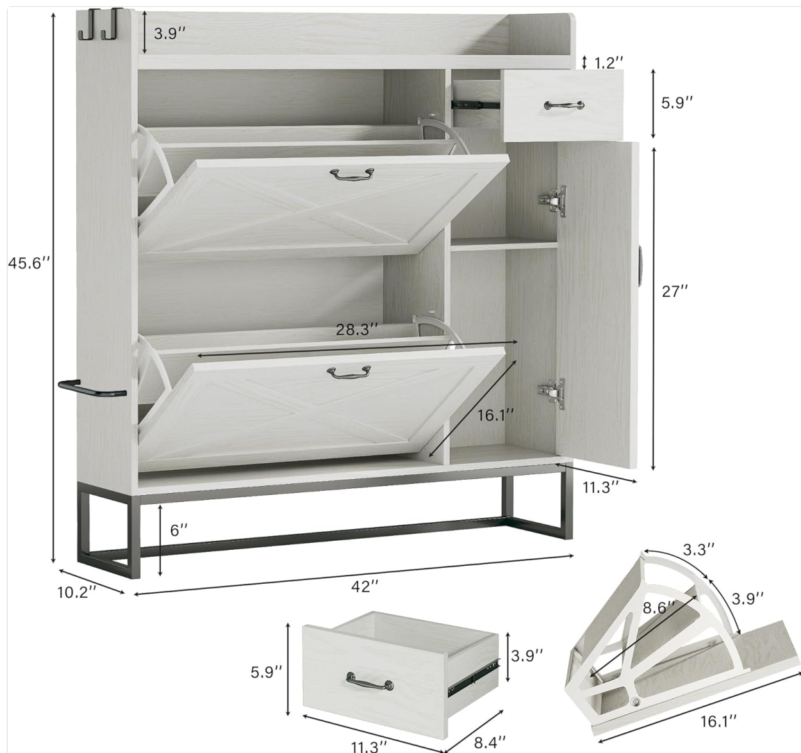
Figure 1: Product Dimensions. This diagram illustrates the overall dimensions of the shoe cabinet, including depth, width, and height, along with internal measurements for drawers and compartments.
