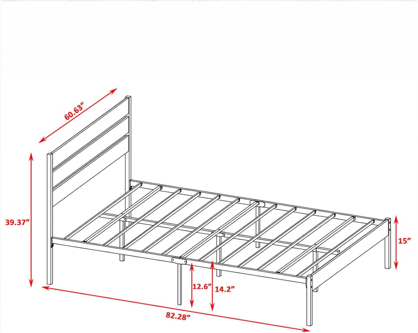
Image: Dimensional diagram of the bed frame.
